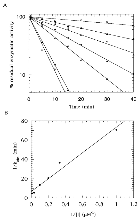
Figure 2. (A) Time course of inactivation of cathepsin B by Cbz-Phe-O-Bn-Thr-epoxide, in 80 mM phosphate buffer, containing 10% (v/v) acetonitrile, 0.5 mM DTT, and 2 mM EDTA, at 25 °C. Inhibitor concentration: (○) 0 μM; (●) 1 μM; (◇) 3 μM; (◆) 5 μM; (△) 10 μM; (▲) 30 μM; (□) 100 μM. (B) Replot of 1/k_{\text{obs}} vs 1/[I] .
